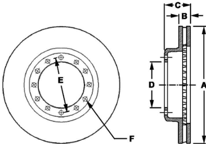
Rotor Configuration
